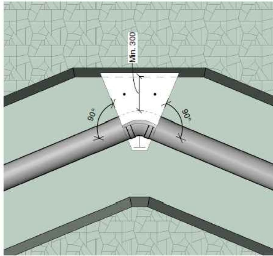
PLAN
